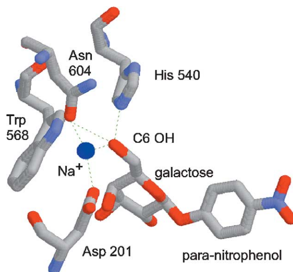
Figure 1. Structure of the Escherichia coli \beta -galactosidase active site. 30 The para -nitrophenyl- \beta -D-fucopyranoside (“novel substrate”) is identical with para -nitrophenyl- \beta -D-galactopyranoside (“native substrate”, shown here), except that it lacks the C6 hydroxyl group. The dotted lines represent hydrogen bonds. The Asp201, His540, and Asn604 residues were “randomized” in this study. The sodium ion (blue sphere) is reduced in scale so as not to obscure these amino acid residues.
