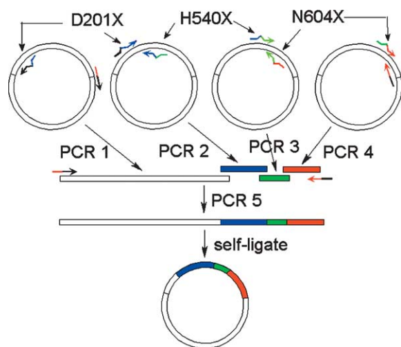
Figure 2. Randomization of \beta -galactosidase residues 201, 540 and 604. Complementary primer pairs (arrows) encoding vector sequence (black) or lacZ (colored) were synthesized. The lacZ -specific primers were degenerate (NNK) at codons 201, 540 and 604. The 6his- lacZ -pET28a+ (white circle) was employed as a template in four separate PCR reactions (white bar = vector–201, blue bar = 201–540, green bar = 540–604, red bar = 604–vector). Each PCR product overlapped one or two others in sequence; the four PCR products were combined in a single overlap PCR reaction (reaction 5). The full-length recombinant PCR product was purified, self-ligated and electroporated into E. coli .
