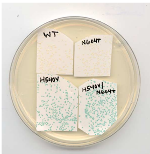
Figure 3. E. coli colonies expressing evolved \beta -fucosidases. E. coli DH5 \Delta lac(DE3) were transformed with the ancestral, H540V, N604T or H540V/N604T variants of the 6his- lacZ -pET28a+ plasmid. The colonies were propagated on LB-kanamycin agar plates, adsorbed to nitrocellulose filters and transferred colony-site up to LB-kanamycin agar plates supplemented with 0.5 mM IPTG and 80 micrograms/ml X-fuc. This photograph was taken 90 minutes after induction.
