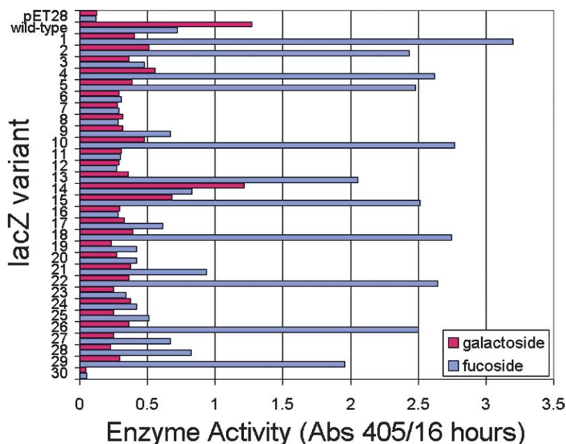
Figure 4. The \beta -galactosidase and \beta -fucosidase activities of selected lacZ variants. E. coli cells were transformed with mutated 6his- lacZ -pET28a+ plasmids (or with the ancestral or no insert control plasmids), grown to mid-log stage in LB-kanamycin liquid cultures, and induced for 3 hours with 0.5 mM IPTG. Each culture was split and reacted with either 0.5 mM para -nitrophenyl- \beta -D-galactopyranoside (native substrate, red) or para -nitrophenyl- \beta -D-fucopyranoside (novel substrate, blue). The formation of the para -nitrophenol product was monitored continuously in a microplate spectrophotometer for 16 h.
